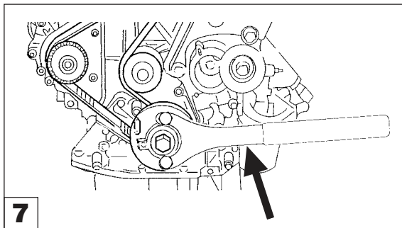
4576 Repositioning Tool
