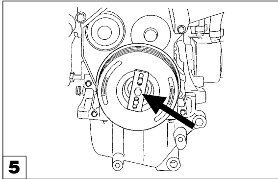
4566 Crank Pulley Remover
