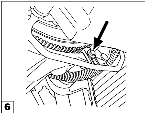
4358 Flywheel Holding Tool (Crank Pulley removal)
