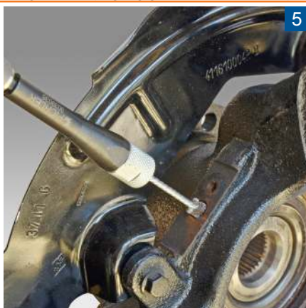
bore for the ABS sensor
